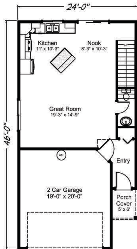
Avalon 1593 sq. ft. • 3 bedrooms • 2 1/2 baths • 2 car garage
