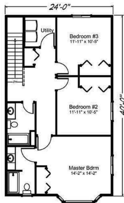
Avalon 1593 sq. ft. • 3 bedrooms • 2 1/2 baths • 2 car garage
