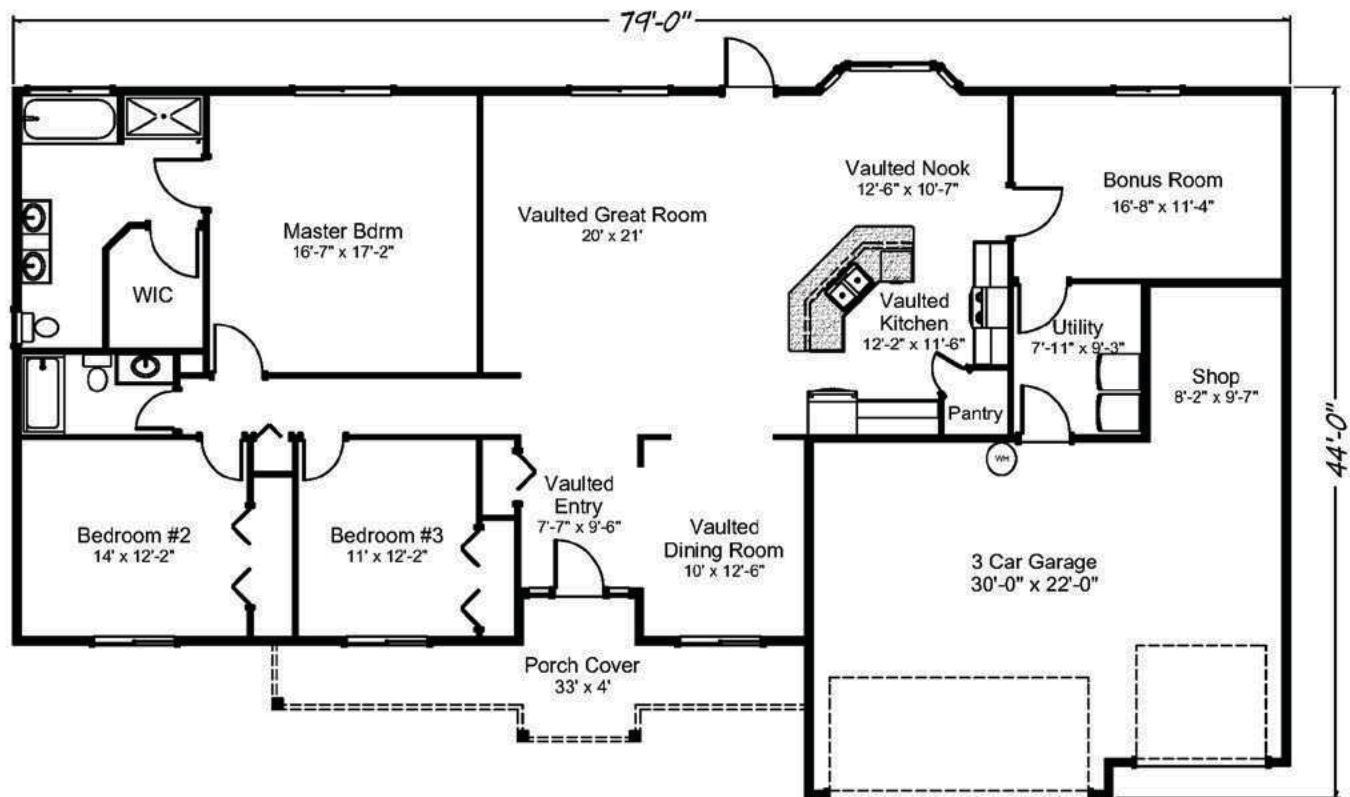
Riverside 2261 sq. ft. • 3 bedrooms • 2 baths • 3 car garage
