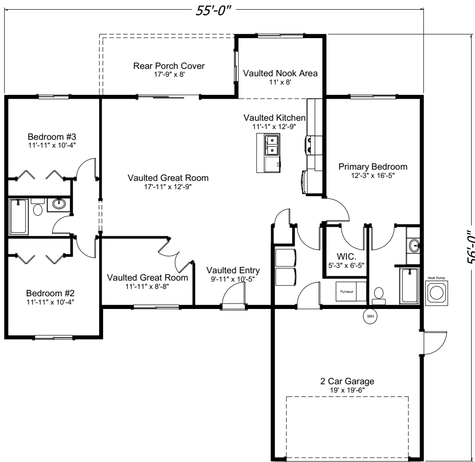
Aspen Lakes 1687 sq. ft. • 3 bedrooms • 2 bath • 2 car garage
